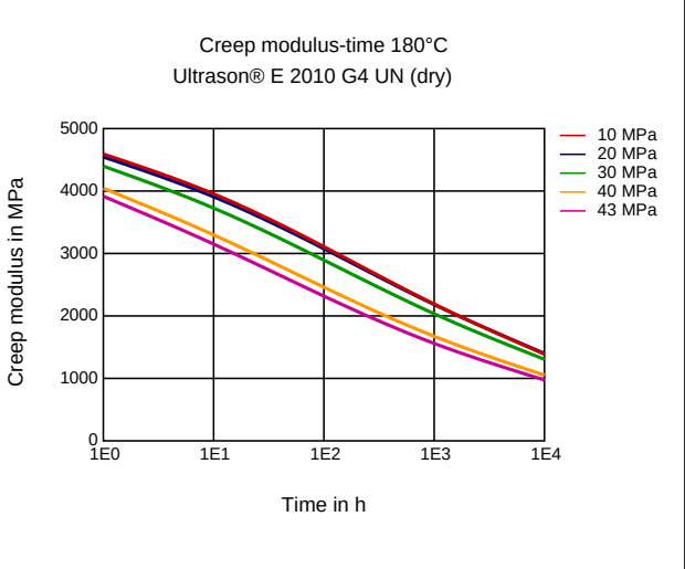
Creep modulus-time 180 °C
